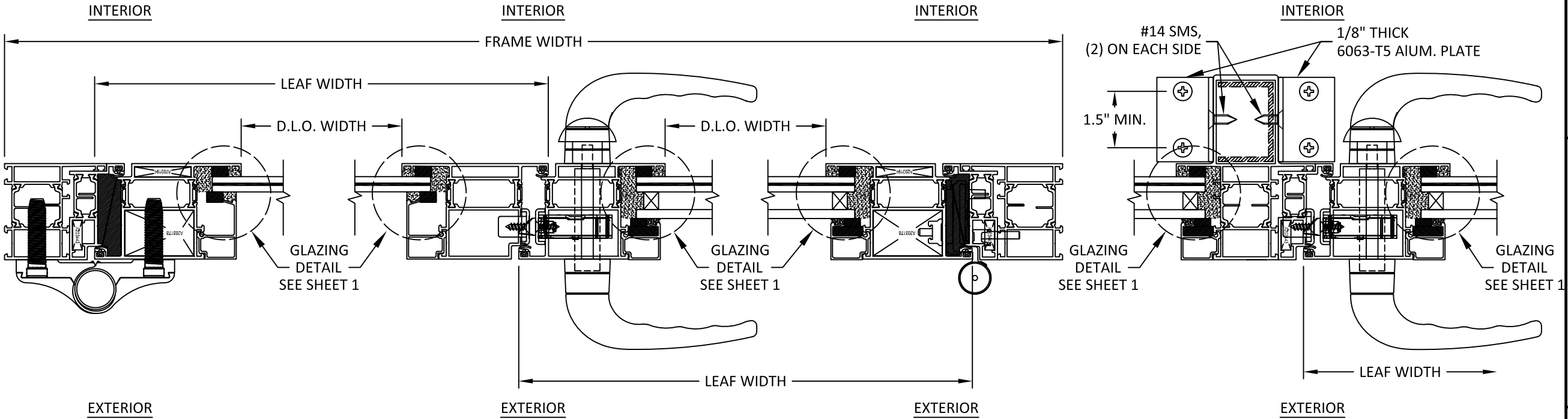
F HORIZONTAL SECTION INACTIVE HINGE JAMB G HORIZONTAL SECTION ASTRAGAL H HORIZONTAL SECTION ACTIVE HINGE JAMB I HORIZONTAL SECTION LOCK MULLION
