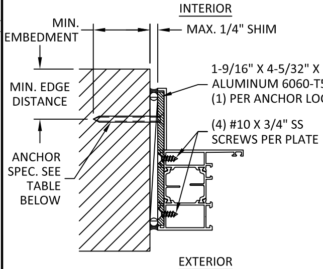
N7 INSTALLATION DETAIL INSTALLATION PLATE DOOR & SIDELITE
