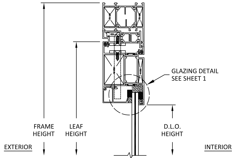
A 5 VERTICAL SECTION DOOR HEAD
