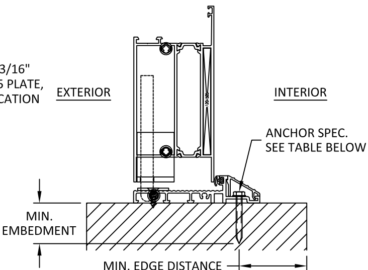
Q7 INSTALLATION DETAIL DOOR SILL - OPTION 1
