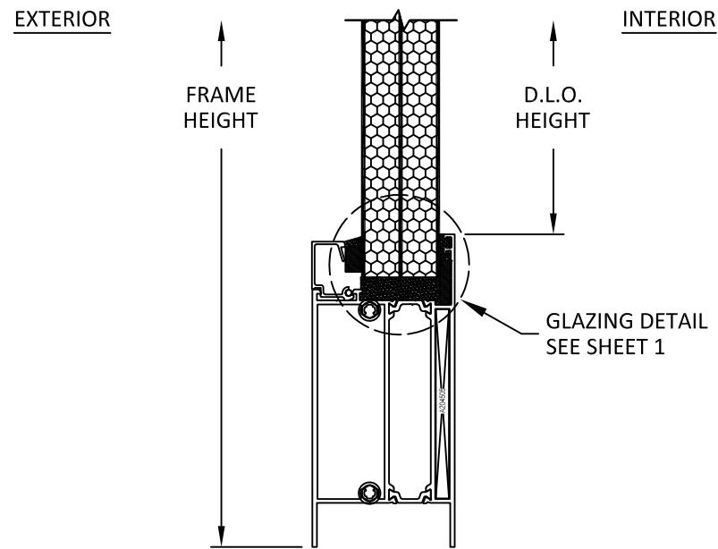
E 5 VERTICAL SECTION SIDELITE SILL NO ANCHOR TO SUBSTRATE
