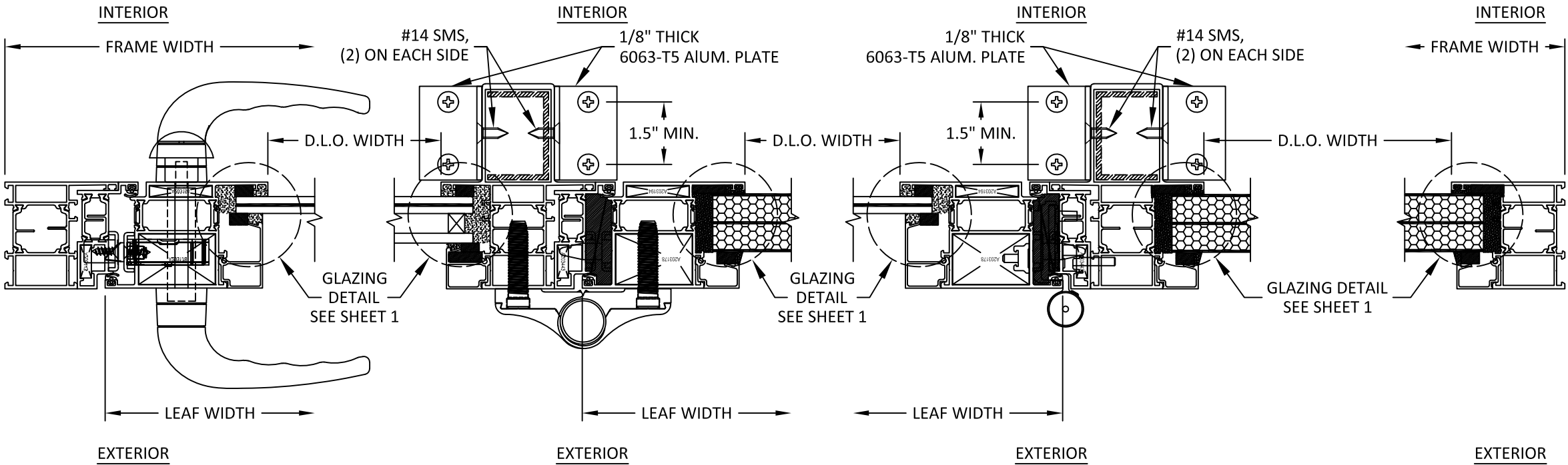
J HORIZONTAL SECTION LOCK JAMB K HORIZONTAL SECTION INACTIVE HINGE MULLION L HORIZONTAL SECTION ACTIVE HINGE MULLION M HORIZONTAL SECTION SIDELITE JAMB
