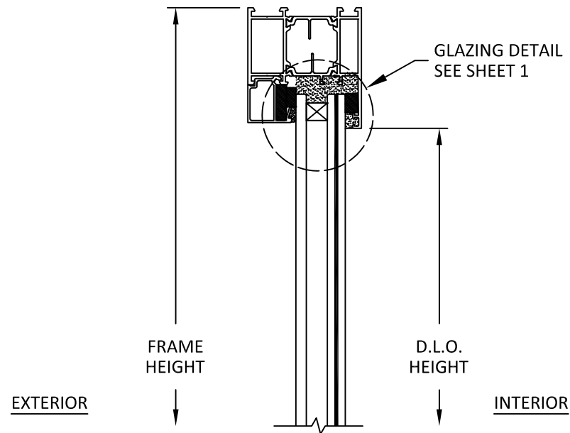
D 5 VERTICAL SECTION SIDELITE HEAD
