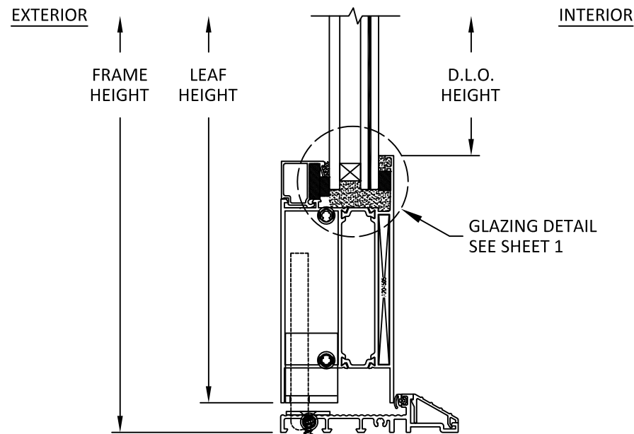
B 5 VERTICAL SECTION DOOR SILL OPTION 1
