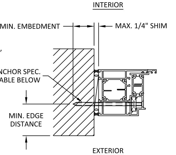
O7 INSTALLATION DETAIL THROUGH FRAME DOOR
