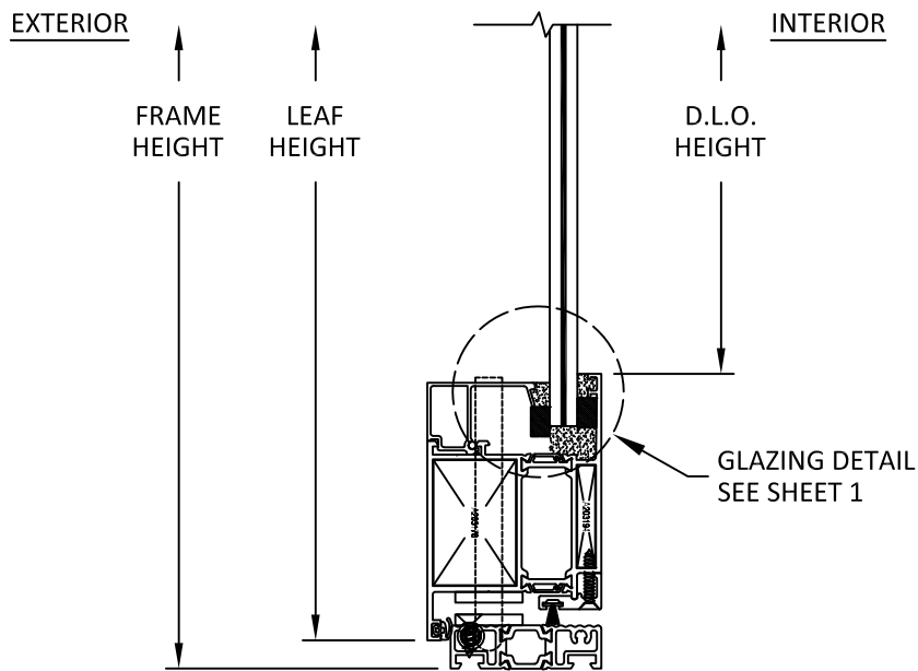
C 5 VERTICAL SECTION DOOR SILL OPTION 2
